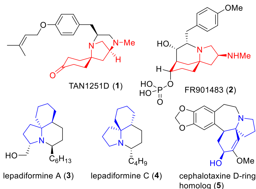
Figure 1. Alkaloids with spiro[cyclohexane-pyrrolidine] core
