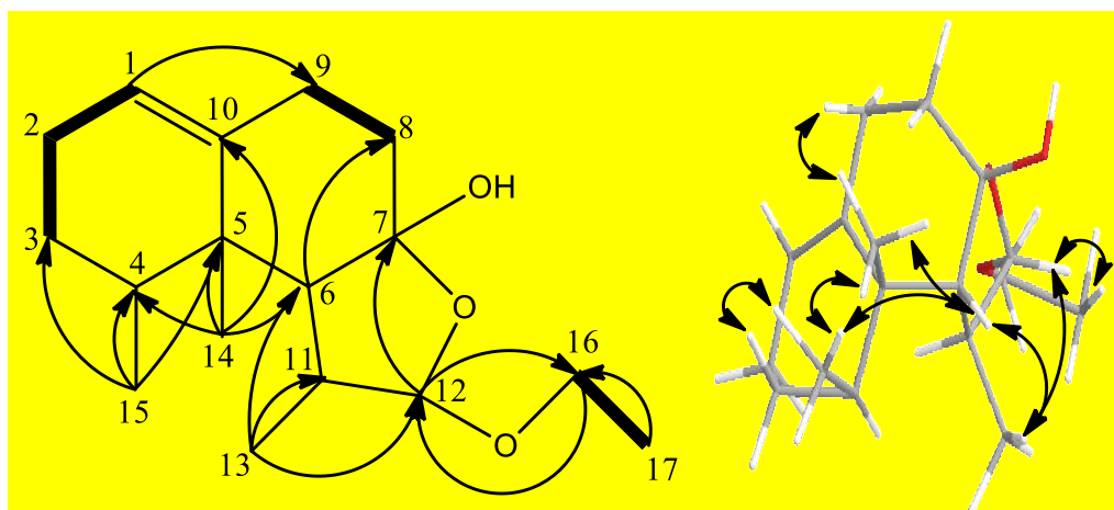
Scheme 2. The key ^1\text{H} - ^1\text{H} COSY (bold lines) and selective HMBC (single-headed arrows) and NOE (double-headed arrows) correlations of compound 1
