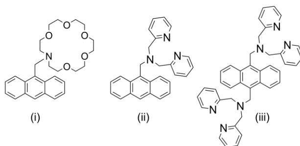
Chart 1. Examples of conventional anthracene-based fluorescent PET probes
