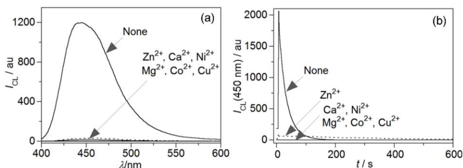
Figure 3. (a) Effects of metal cations ( 1.0 \times 10^{-2} M) on the CL spectra of cyclic-hydrazide 2 ( 5.0 \times 10^{-5} M) in DMSO in the presence of \text{H}_2\text{O}_2 ( 5.0 \times 10^{-2} M), \text{Bu}_4\text{NOH} ( 5.0 \times 10^{-2} M), \text{KI} ( 2.5 \times 10^{-2} M), and metal cations ( 1.0 \times 10^{-2} M). The CL spectra were recorded 10 s after the CL reaction started. Dotted line shows CL spectrum observed in the presence of \text{Zn}^{2+} . (b) Time profiles of the CL of cyclic-hydrazide 2 observed at \lambda_{\text{CL}} 450 nm. Dotted line shows CL profile observed in the presence of \text{Zn}^{2+} .
