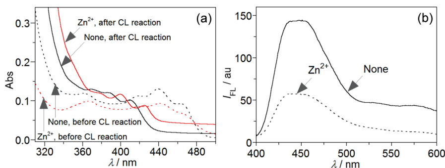
Figure 5. (a) Absorption spectra of the CL mixture of cyclic-hydrazide 2 ( 5.0 \times 10^{-5} M) in DMSO in the presence \text{H}_2\text{O}_2 ( 5.0 \times 10^{-2} M), \text{Bu}_4\text{NOH} ( 5.0 \times 10^{-4} M). Dotted lines: Before the CL reaction. Solid lines: After the CL reaction upon addition of KI ( 2.5 \times 10^{-5} M). (b) Fluorescence spectra ( \lambda_{\text{ex}} 350 nm) of the CL reaction mixture of cyclic-hydrazide 2 .
