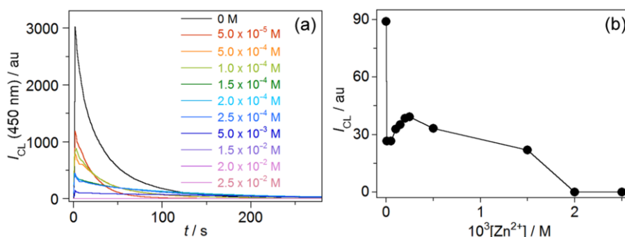
Figure 4. (a) Time profiles of chemiluminescence emission of compound 2 in the presence of \text{Zn}^{2+} . (b) Relative CL intensity plotted as a function of [\text{Zn}^{2+}] : [\mathbf{2}] = 5.0 \times 10^{-5} M, [\text{M}^{2+}] = 2.0 \times 10^{-2} M, [\text{H}_2\text{O}_2] = 5.0 \times 10^{-2} M, [\text{Bu}_4\text{NOH}] = 5.0 \times 10^{-2} M, [\text{KI}] = 2.5 \times 10^{-2} M.
