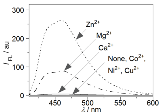
Figure 1. Effects of metal cations (10 equiv.) on the FL spectra ( \lambda_{\text{ex}} 403 nm) of carboximide 1 ( 1.0 \times 10^{-5} M) in MeCN
