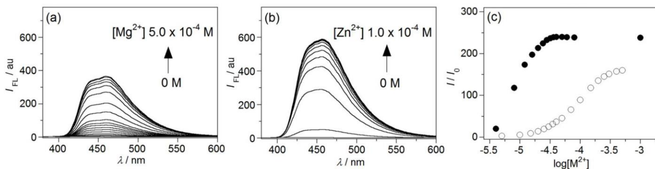
Figure 2. Effects of \text{Mg}^{2+} and \text{Zn}^{2+} on the FL spectra of carboximide 1 ( 1.0 \times 10^{-5} M) in MeCN. (a) \text{Mg}^{2+} ( 0 – 5.0 \times 10^{-4} M, \lambda_{\text{ex}} 350 nm), (b) \text{Zn}^{2+} ( 0 – 1.0 \times 10^{-4} M, \lambda_{\text{ex}} 363 nm). (c) FL titration results for \text{Mg}^{2+} at \lambda_{\text{FL}} 456 nm ( \circ ) and \text{Zn}^{2+} at \lambda_{\text{FL}} 445 nm ( \bullet ).
