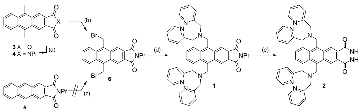
Scheme 1. Synthetic routes to DPAM-modified carboximide 1 and cyclic-hydrazide 2 . Reagents and conditions: (a) PrNH 2 , toluene, reflux, 15 h, then Ac 2 O, heat, 62%; (b) NBS, BPO, CCl 4 , reflux, 16 h, 96%; (c) (CH 2 O) n , HBr, AcOH, reflux; (d) dipicolylamine, KI, DMF, rt, 1 h, 36%; (e) hydrazine hydrate, EtOH, reflux, 21 h, 44%.
