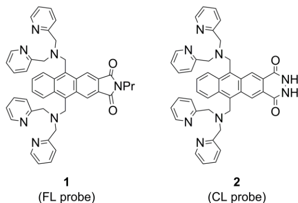
Chart 2. Structures of carboximide 1 and cyclic-hydrazide 2
