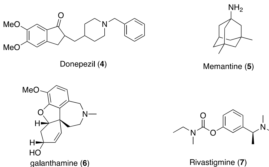
Figure 4. Chemical structures of donepezil (4), memantine (5), galanthamine (6) and rivastigmine (7)
