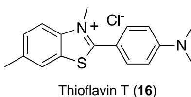
Figure 6. Chemical structure of thioflavin T ( 16 )
