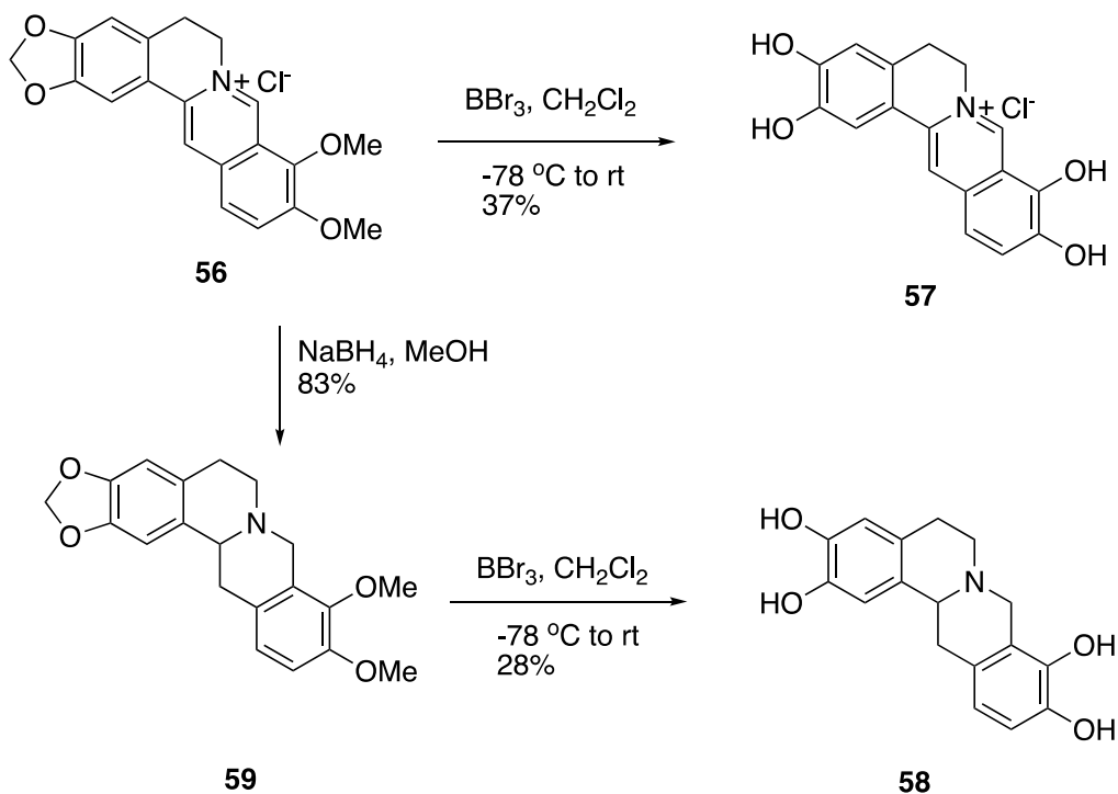
Scheme 7. Synthesis of berberine analogues 57 and 58
