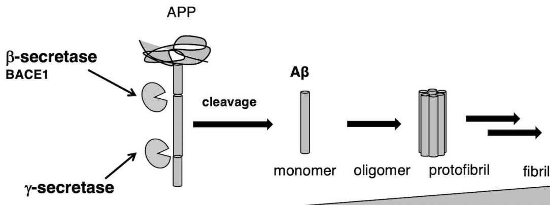
Figure 2. The formation of amyloid fibrils by the synthesis and aggregation of A \beta 42
