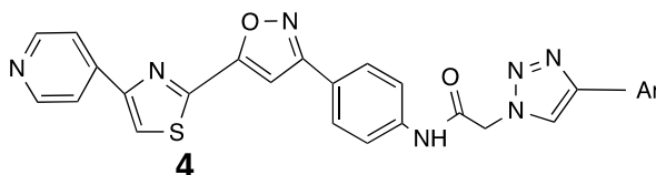
4a ; Ar =3,4,5-trimethoxyphenyl 4b ; Ar =4-chlorophenyl 4c ; Ar =4-nitrophenyl
