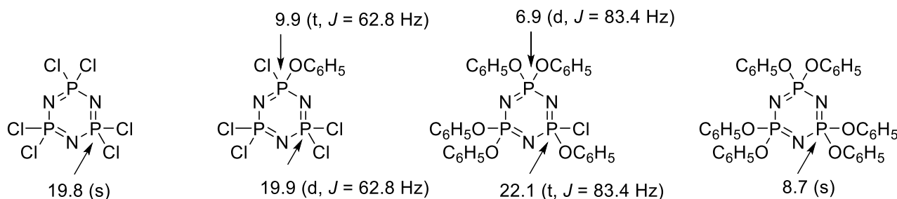
Figure 2. ^{31}\text{P} NMR of cyclotriphosphazene derivatives
