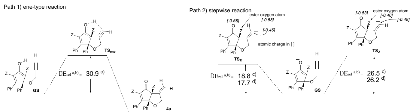
Figure 6. Calculated atomic charge and reaction barriers of the two possible reaction pathways of 1a and 2a
