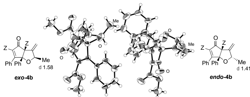
Figure 2. X-Ray structures of exo - 4b and endo - 4b involved in the asymmetric unit of the co-crystal and the ^1\text{H} NMR chemical shifts of methyl groups
