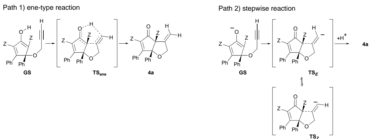
Scheme 4. Possible reaction pathways
