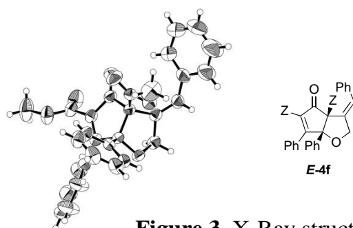
Figure 3. X-Ray structure of E - 4f
