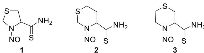
Figure 1. Structures of the alicyclic N -nitrosamines
