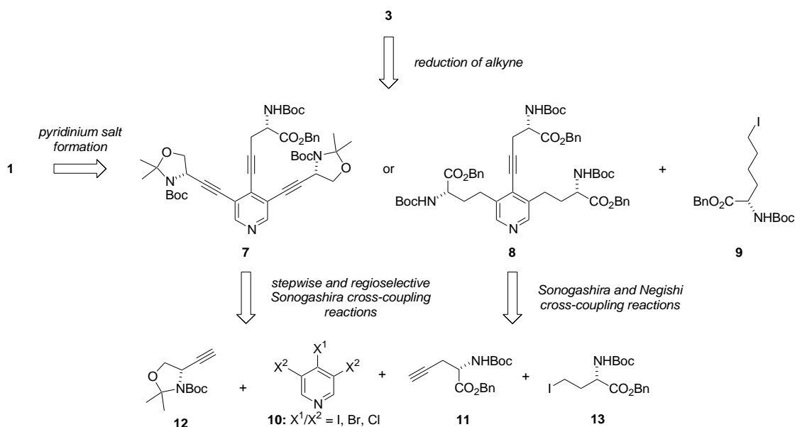
Scheme 1. Retrosynthetic analysis of desmosine ( 1 ) and desmopyridine ( 3 )
